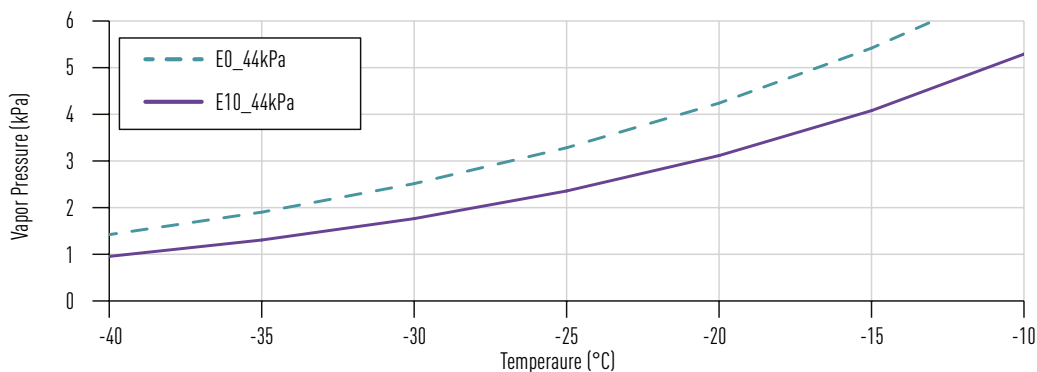
Figure G-38: Magnification of Figure G-37 at Temperatures Below Freezing
