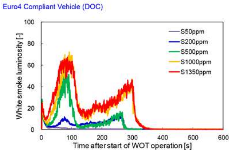
Figure DF-16: White Smoke Luminosity at Different Sulphur Levels
