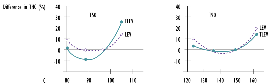
Figure G-35: Effect of T50/T90 on Exhaust Emissions, Comparison of LEV and TLEV
