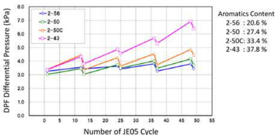
Figure DF-29: Influence of Total Aromatics Content on DPF Differential Pressure
